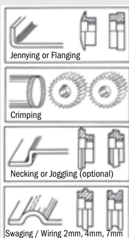
Standard wheels - SJ2
